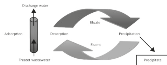
Process principle of further phosphorus removal from municipal wastewater in combination with phosphorus recovery
